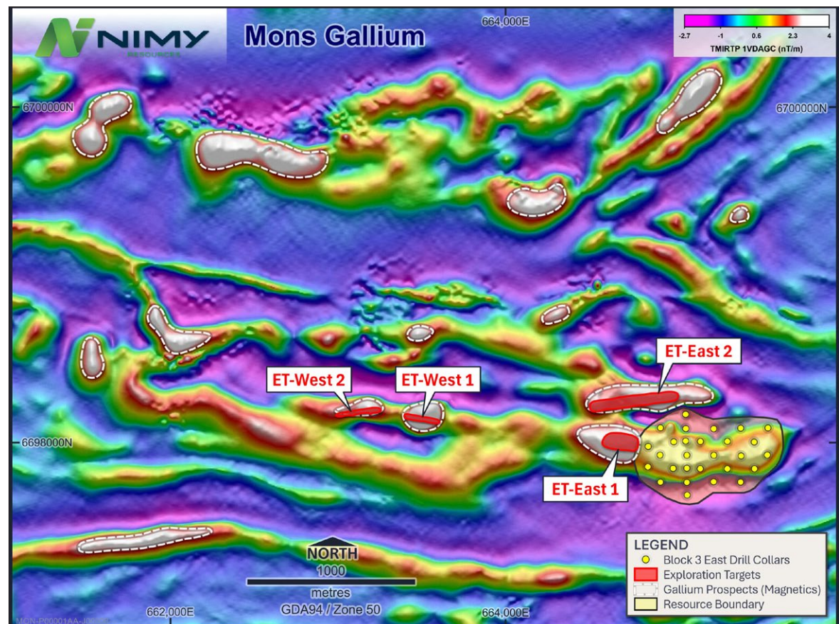
Exploration targets and first priority targets, along extended 3.5km host rock unit. (ASX Announcement 03/02/26)
