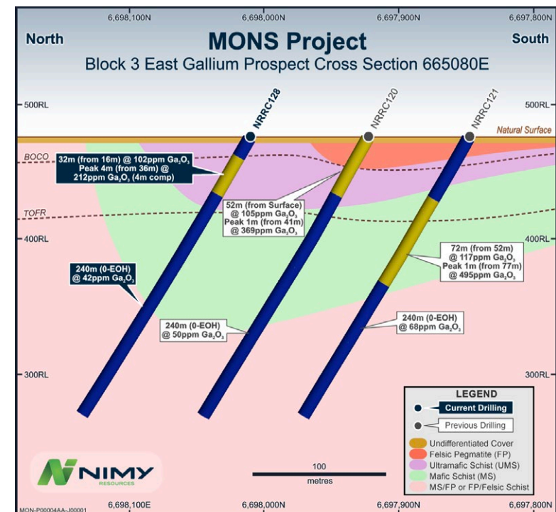
Schematic cross section view of Block 3 East Gallium Prospect looking east. (ASX Announcement 09/10/24)
